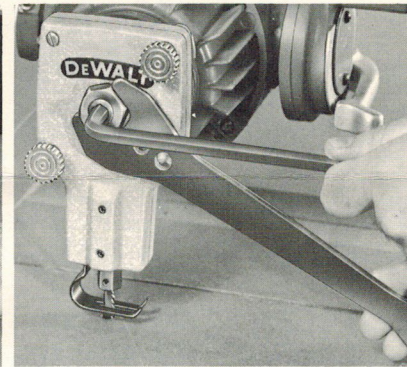
MOUNTS DIRECTLY ON MOTOR
