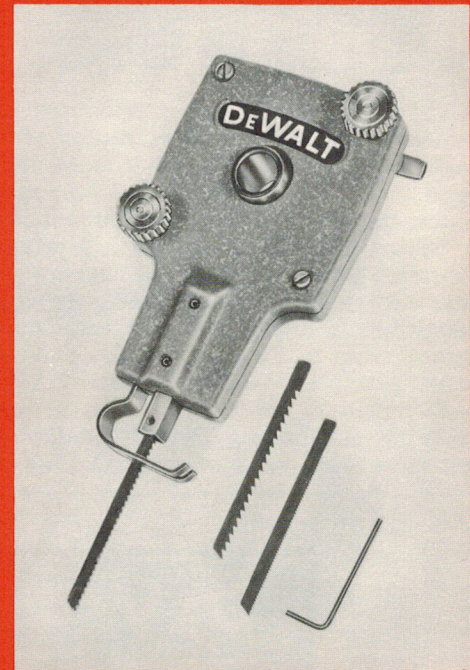
MOUNTS DIRECTLY ON MOTOR
