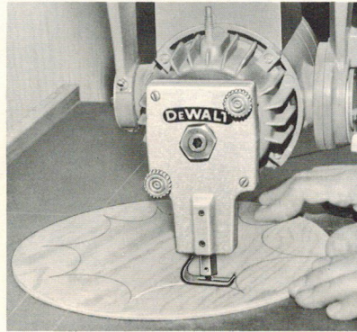
DOES INSIDE CURVE WORK
