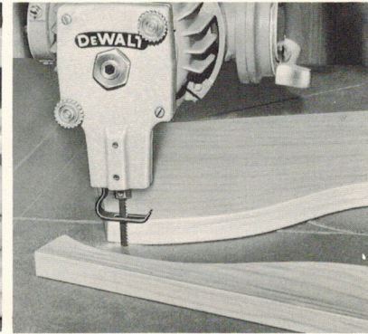
DOES OUTSIDE CURVE WORK
