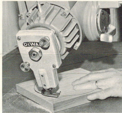
DOES ANGLE CURVE WORK
